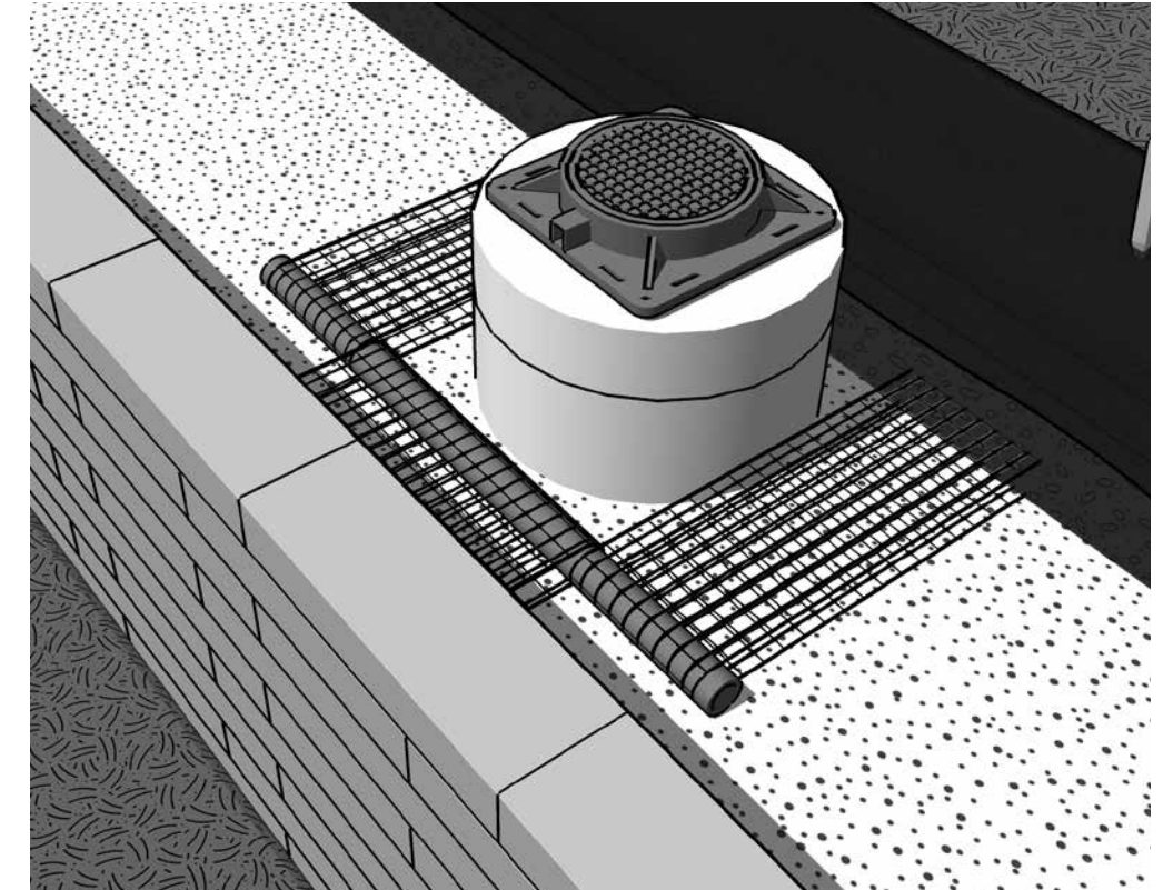
1 CATCH BASIN
