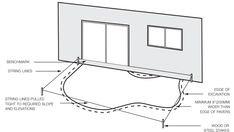
Figure 9. Project layout and staking
