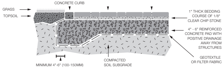
Figure 6. Paver installation over cast-in-place concrete
