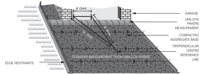
Figure 17. Edge restraint positioning.
