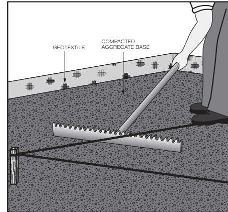
Figure 15. Use a grading rake for checking grades
