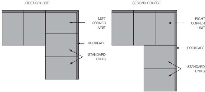
Figure 41. Outside corner typical installation
