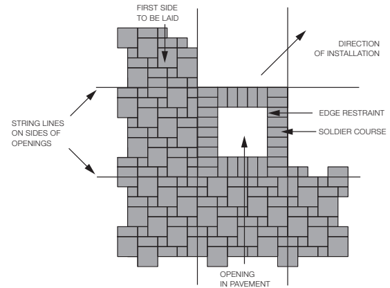
Figure 23. Paving around an opening or obstruction.
