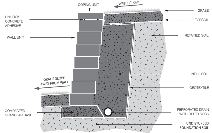
Figure 35. Encapsulate granular backfill and finish grading.
