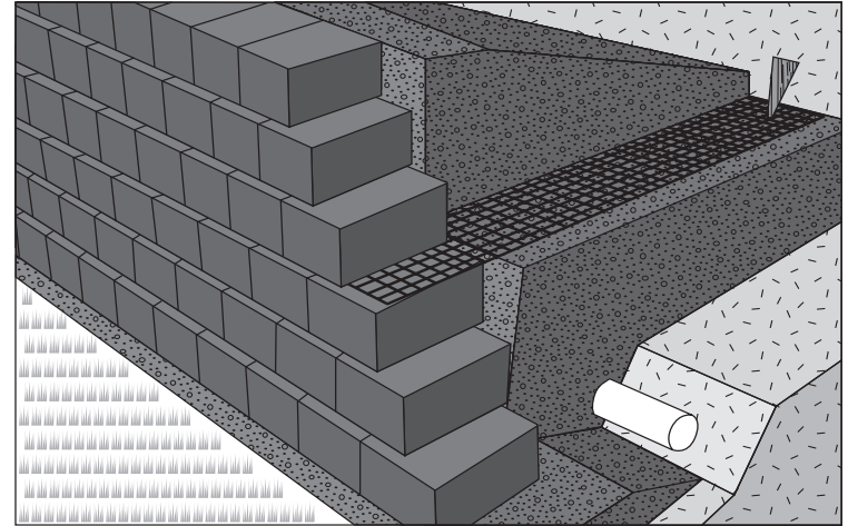
Figure 38. Backfilling over geogrid.
