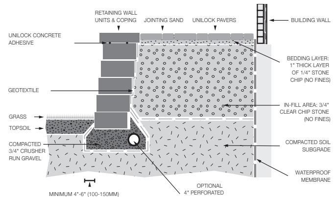
Figure 5. Patio/Terrace installation with wall units and coping
