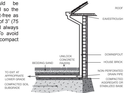
Figure 12. Downspout
