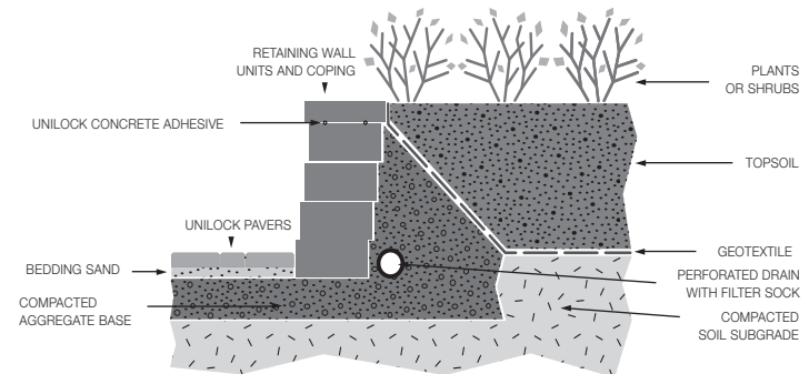
Figure 51. Typical planter application.
