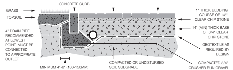
Figure 4. Permeable paver installation with precast or cast-in-place curb unit
