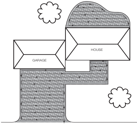
Figure 14. Compaction directions.
