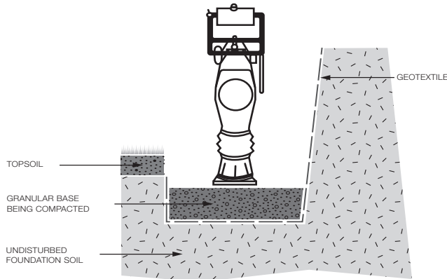
Figure 33. Base compaction
