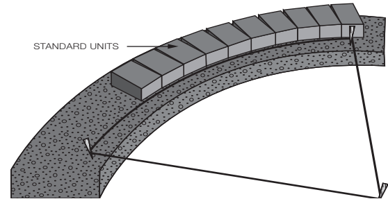
Figure 43. On inside curves, the radius will increase with height.
