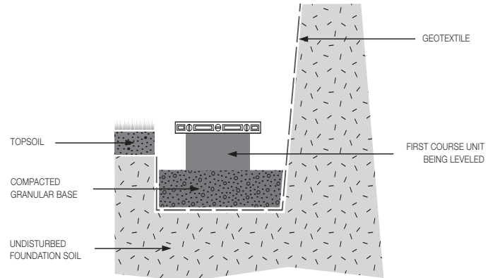
Figure 34. First course positioning and leveling.
