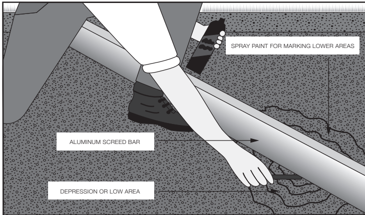
Figure 16. Check grades with a screed bar.
