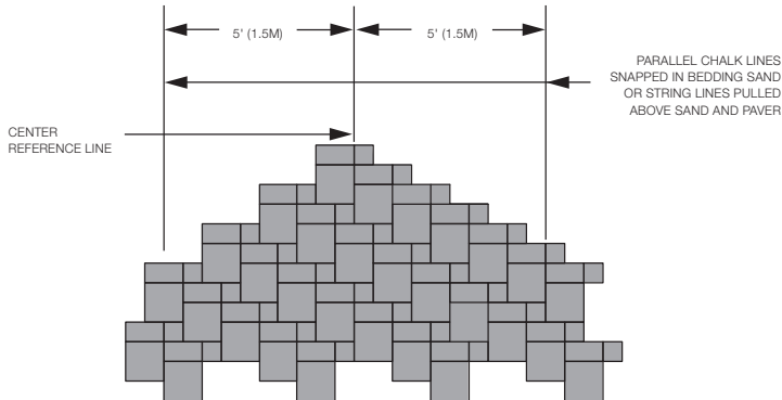
Figure 22. Parallel lines and center reference line.
